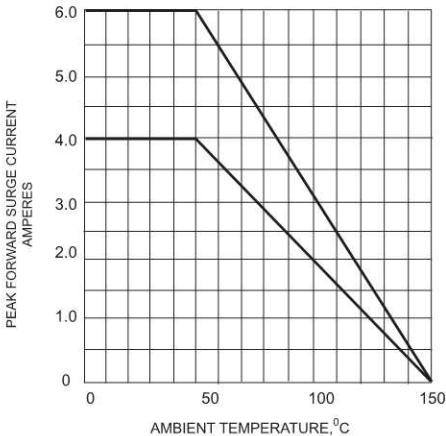
FIG.2 - DERATING CURVE OUTPUT RECTIFIED CURRENT
