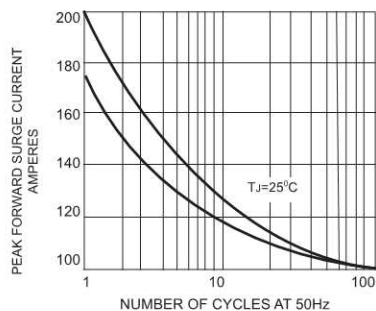
FIG.1 - MAXIMUN FORWARD SURGE CURRENT
